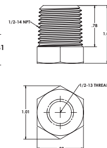
Optional Reducer 1/2-14 NPT - 1/2-13 2-8057
