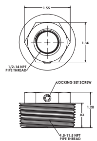
Optional Reducer 1 1/2 - 1/2NPT 2-8059
