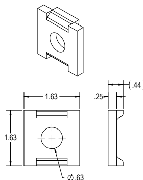
Locking Tab
