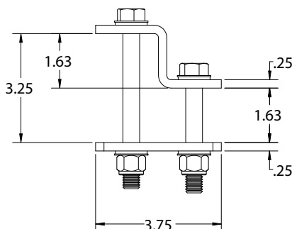
Z Bracket CG-P1045-ZB Side View
